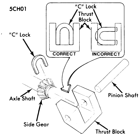
POSITIONING "C" LOCK FOR REMOVAL
