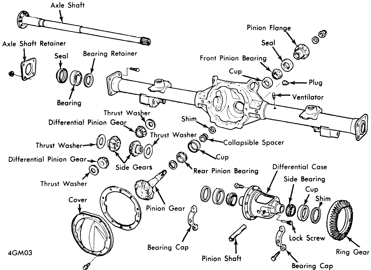
GENERAL MOTORS 8 1/2" & 8 7/8" RING GEAR AXLE ASSEMBLY
