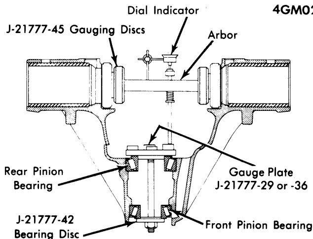
PINION DEPTH TOOL SET J21777 (INSTALLED)
