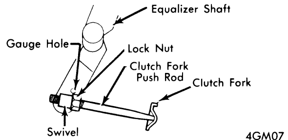
FREE PLAY ADJUSTMENT ("P" MODELS)
