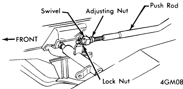
FREE PLAY ADJUSTMENT ("G" MODELS)
