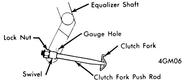
FREE PLAY ADJUSTMENT ("C" & "K" MODELS)
