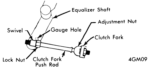
FREE PLAY ADJUSTMENT (P30 W/PROPELLER SHAFT PARKING BRAKE)
