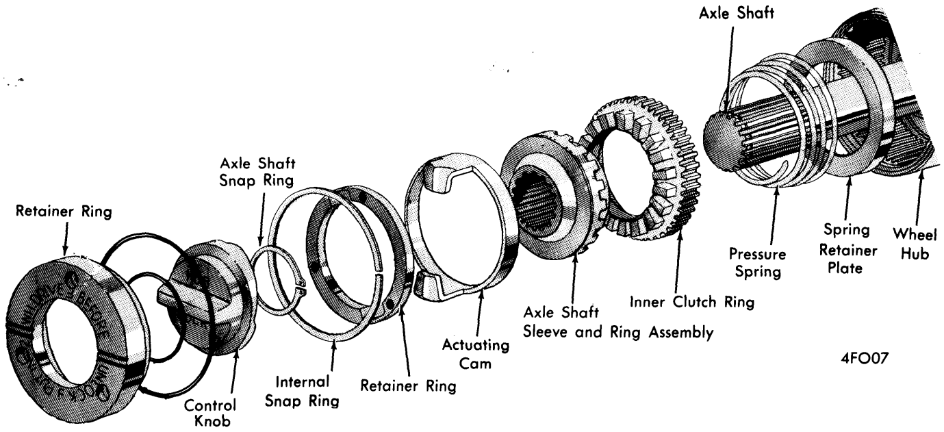
DANA/SPICER LOCKING HUB (THREE BOLT)
