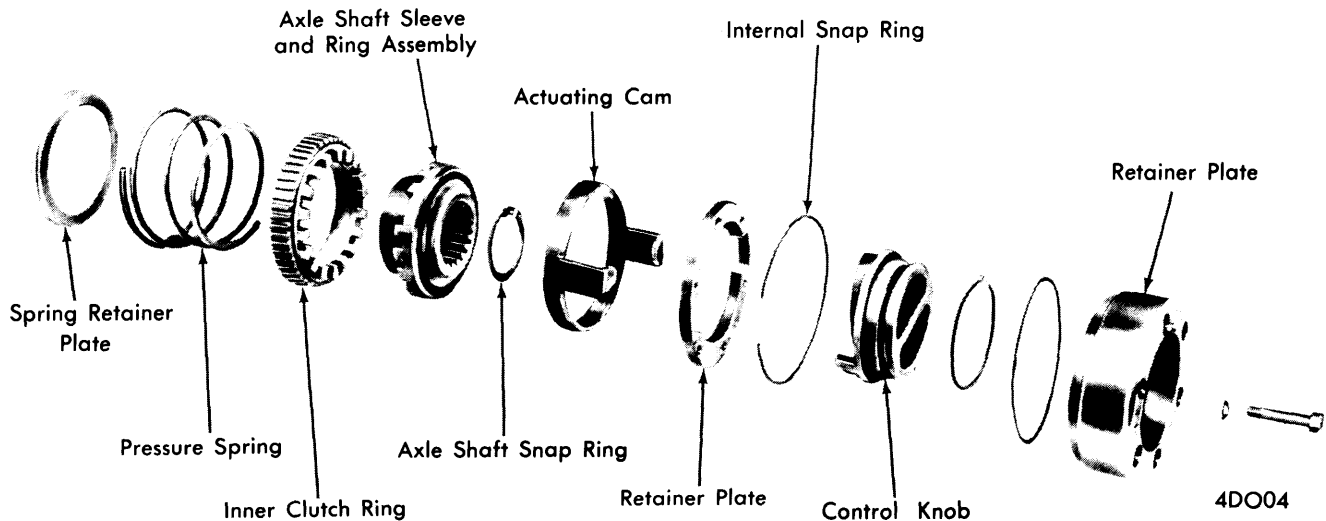
DANA/SPICER LOCKING HUB (SIX BOLT)
