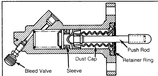
Fig. 3: Sectional View of Clutch Slave Cylinder
