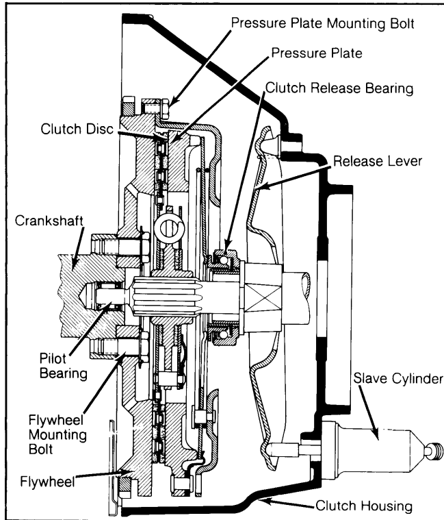
Fig. 1: Typical BMW Clutch Assembly
