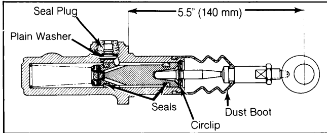
Fig. 2: Sectional View of Clutch Master Cylinder
