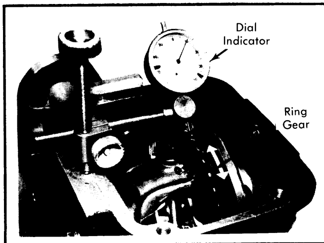
Fig. 7 Checking Ring Gear Backlash
