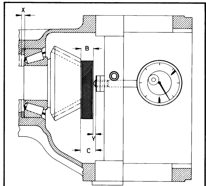
Fig. 4 Pinion Shim Measuring Points
