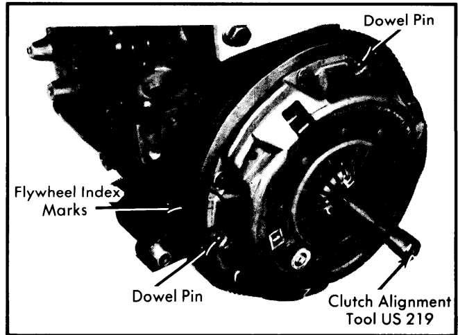
Fig. 2 Aligning Clutch Assembly Reference Marks for Reinstallation
