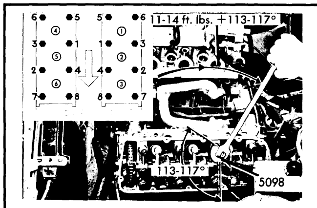
Fig. 3 Final Torquing of Cylinder Head Bolts After Running and Cooling Engine
