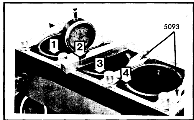
Fig. 12 Checking Liner Height Above Block Face
