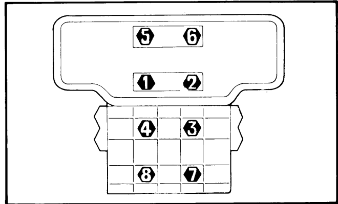
Fig. 9 Tightening Sequence for Main Bearing Nuts
