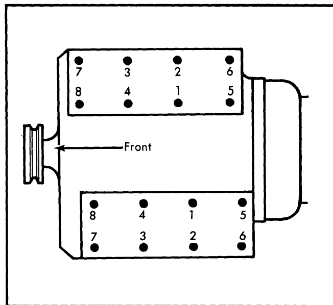
Fig. 4 Cylinder Head Tightening Sequence
