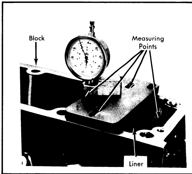
Fig. 8 Measuring Liner Projection
