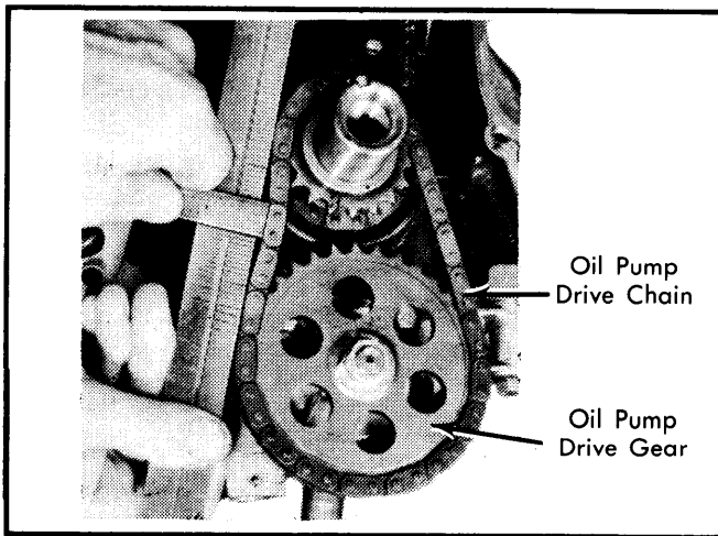
Fig. 4 Measuring Oil Pump Chain Deflection
