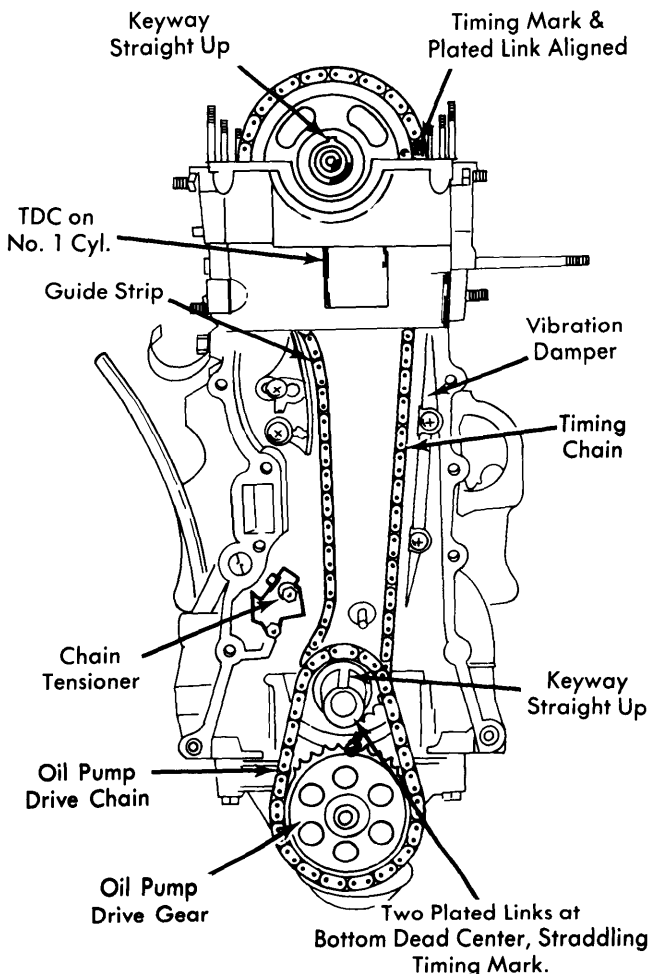
Fig. 2 Timing Chain & Sprocket Alignment
