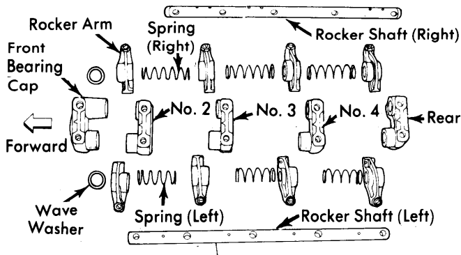
Fig. 10 Exploded View of Rocker Arm and Shaft Assembly (2000 cc Shown; 1600cc and 2600 cc Similar)
