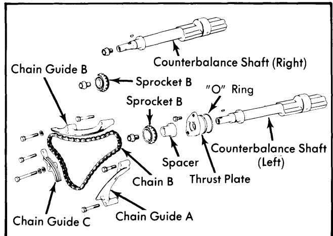
Fig. 5 Exploded View of Counterbalance Shafts and Drive Chain (2000 and 2600 cc)
