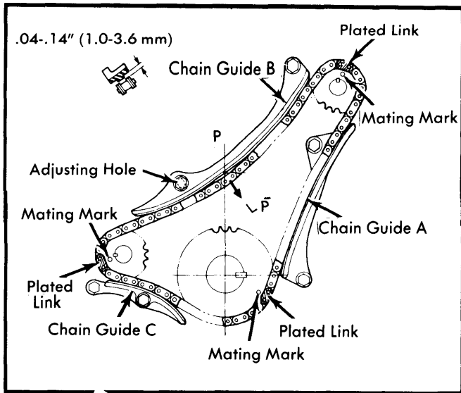
Counterbalance Drive Chain (2000 and 2600 cc)
