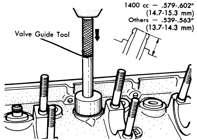
Fig. 11 Valve Guide Installation and Height
