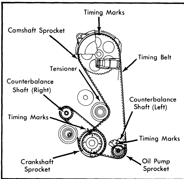
Fig. 4 Counterbalance and Timing Belt Installation (1600 cc)
