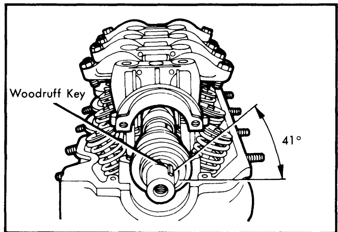
Fig. 8 Camshaft Woodruff Key Position for Installation (1600 cc Engine)
