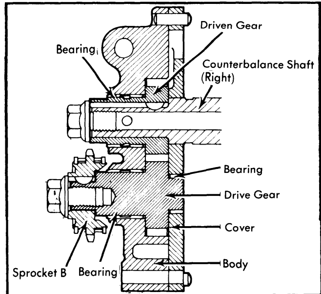
Fig. 14 Cutaway View of Gear Type Oil Pump
