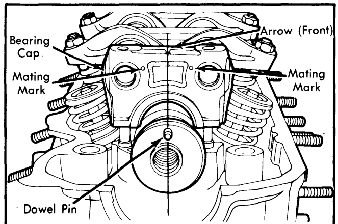
Fig. 9 Camshaft Installation Position and Bearing Cap/Rocker Arm Shaft Mating Marks (2000 and 2600 cc Engines)
