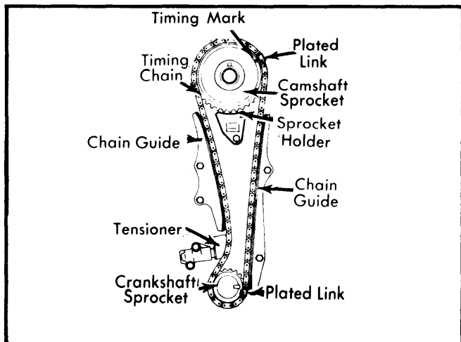
Fig. 7 Camshaft Sprocket Alignment and Installation (2000 & 2600 cc)
