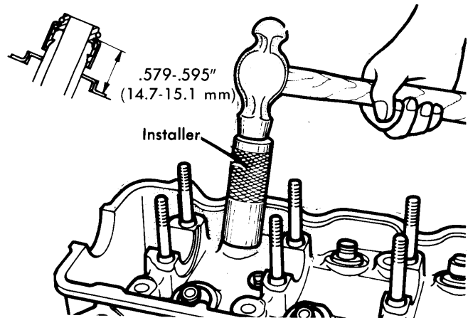
Fig. 12 Valve Stem Oil Seal Installation and Height
