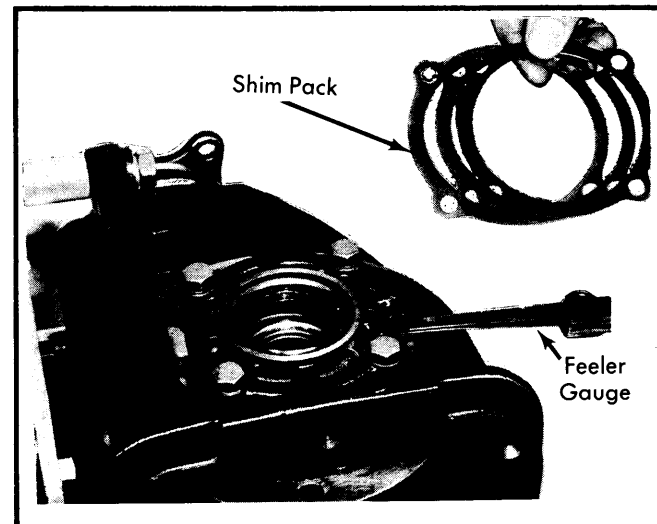
Fig. 6 Measuring for Differential Shim Pack Preload Requirements
