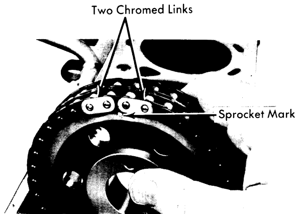
Fig. 10 Aligning Camshaft Sprocket & Timing Chain
