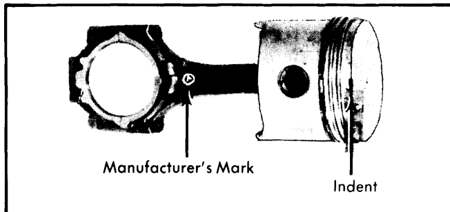
Fig. 7 Correct Alignment of Piston & Rod Assembly
