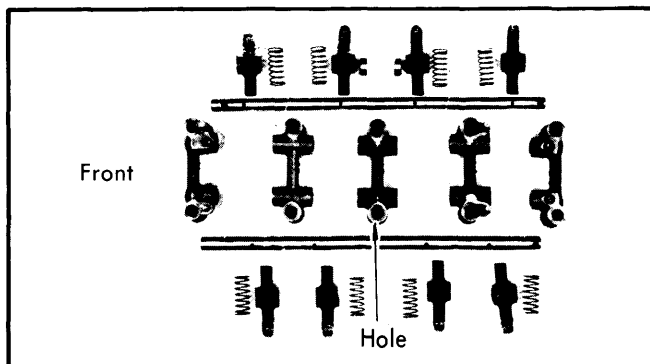
Fig. 3 Disassembled View of Rocker Arm Assembly
