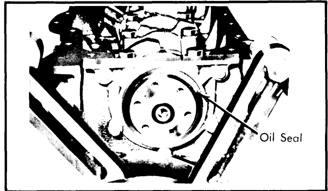
Fig. 8 Installed View of Rear Seal & Retainer
