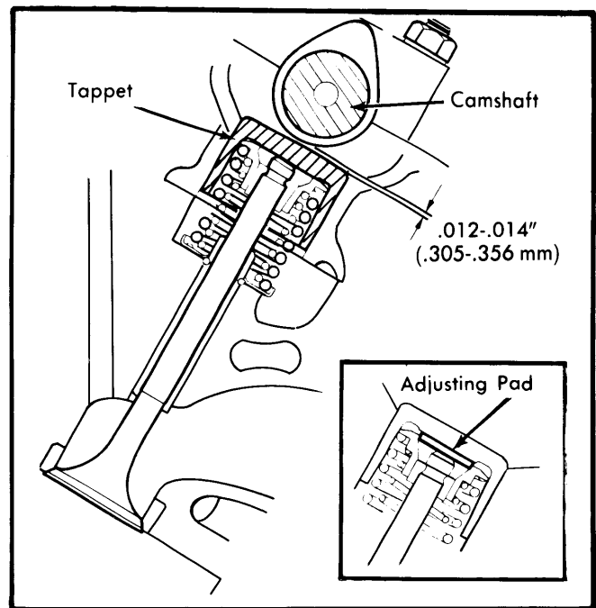
Fig. 5 Correct Valve Tappet Clearance Adjustment Procedure
