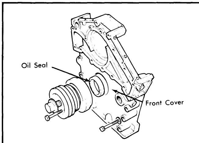
Fig. 8 Detail of Front Cover Oil Seal
