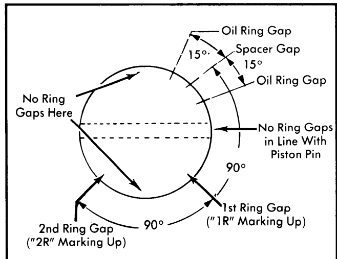
Fig. 2 Piston Ring Installation
