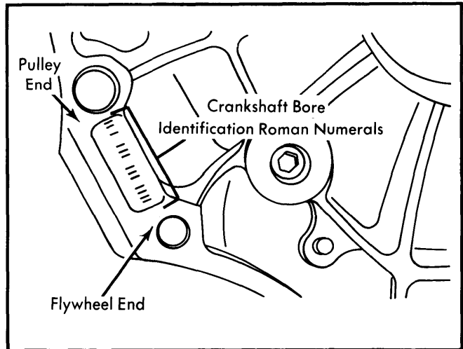
Fig. 3 Crankshaft Identification Locations (All Engines)
