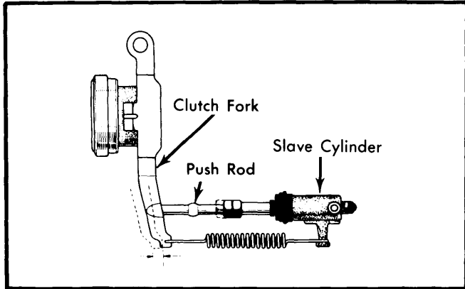
Fig. 5 Clutch Fork Free Play Measurement Location
