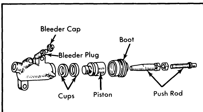
Fig. 3 Exploded View of Slave Cylinder Pickup Cylinder Shown — Other Similar
