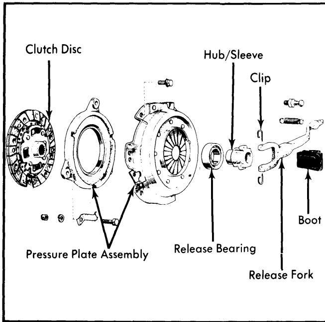
Fig. 1 Exploded View of Typical Clutch Arrangement
