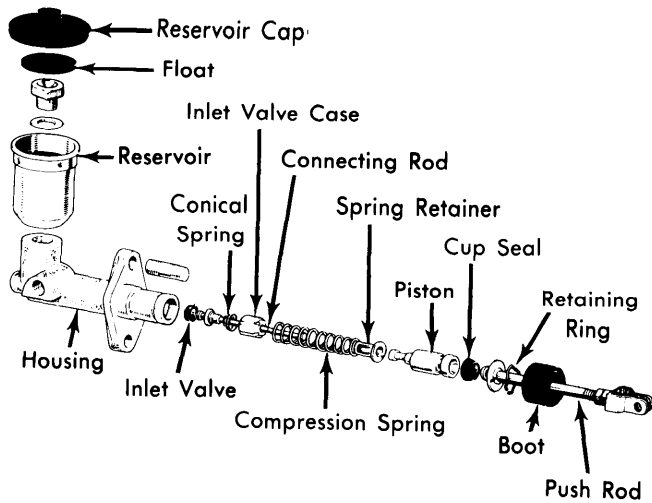
Fig. 2 Exploded View of Clutch Master Cylinder Celica, Corona, Corolla Shown
