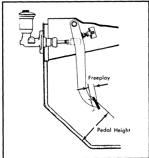
Fig. 4 Pedal Height and Free Play Measuring Points
