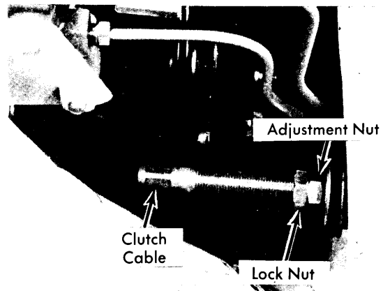
Fig. 2 Clutch Free Play Adjustment Location – Adjustment Nut Moves Along Threaded Rod
