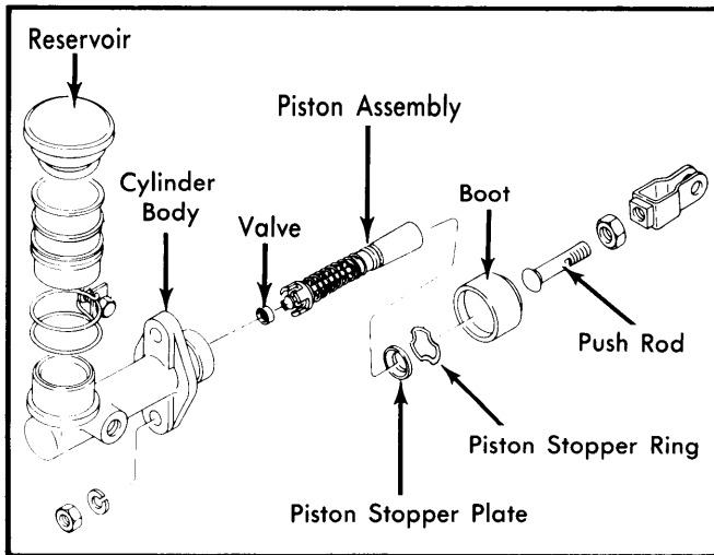
Fig. 3 Exploded View of Master Cylinder
