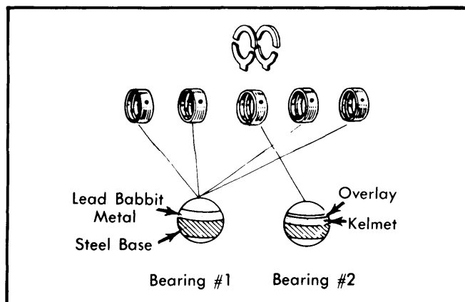
Fig. 9 Crankshaft Bearings
