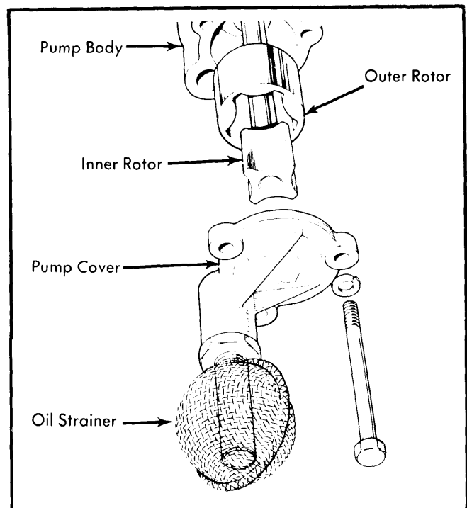
Fig. 4 Engine Oil Pump Disassembled View
