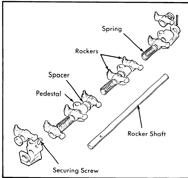
Fig. 2 Disassembled View of Rocker Arm & Shaft
