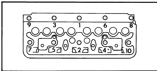
Fig. 1 Midget Cylinder Head Tightening Sequence
