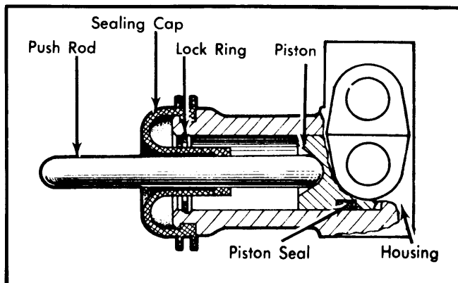
Fig. 3 Sectional View of Clutch Slave Cylinder
