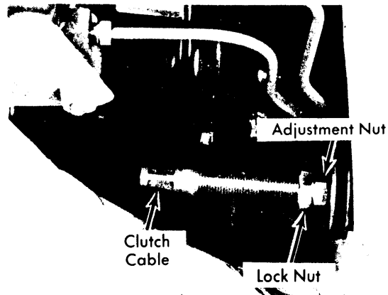
Fig. 2 Clutch Free Play Adjustment Point
