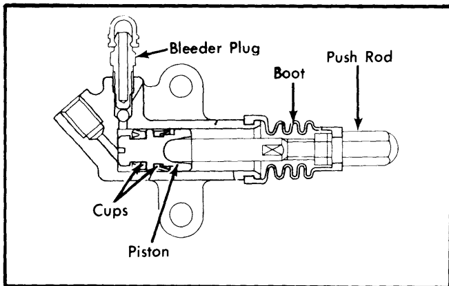
Fig. 3 Sectional View of Adjustable Slave Cylinder
