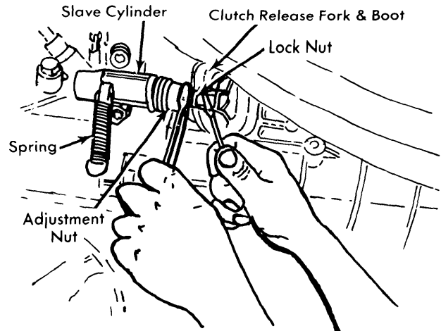
Fig. 6 Making Clutch Release Fork Free Play Adjustment
