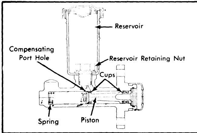
Fig. 2 Clutch Master Cylinder Components (RX4 Model Shown)
