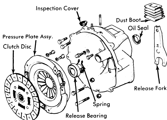
Fig. 1 Exploded View of Cosmo Clutch Assembly
