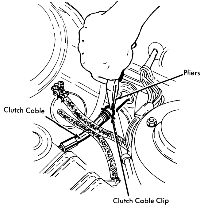
Fig. 3 Clutch Pedal Adjustment Point for CVCC
