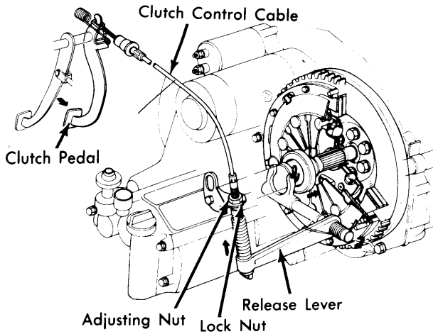
Fig. 2 Clutch Adjustment Point for Civic
