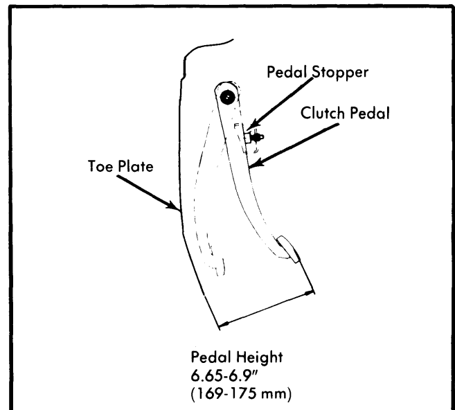
Fig. 5 Pedal Height and Free Play Adjustment
