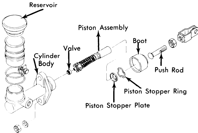
Fig. 3 Exploded View of Master Cylinder
