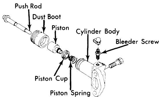
Fig. 4 Exploded View of Clutch Slave Cylinder
