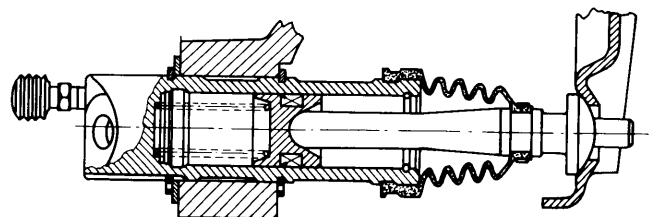
Fig. 3 Sectional View of Clutch Slave Cylinder
