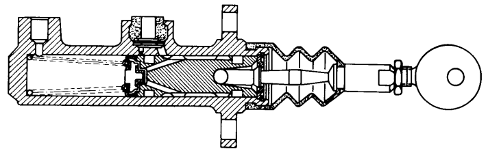
Fig. 2 Sectional View of Clutch Master Cylinder
