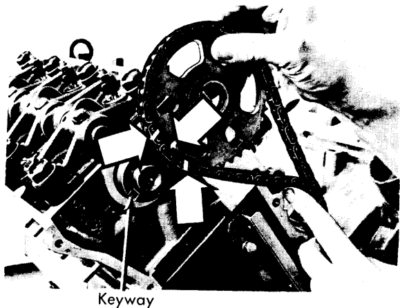
Fig 11 Right Camshaft Keyway and Timing Marks
