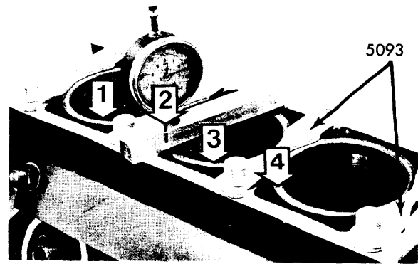
Fig. 10 Checking Liner Height Above Block Face
