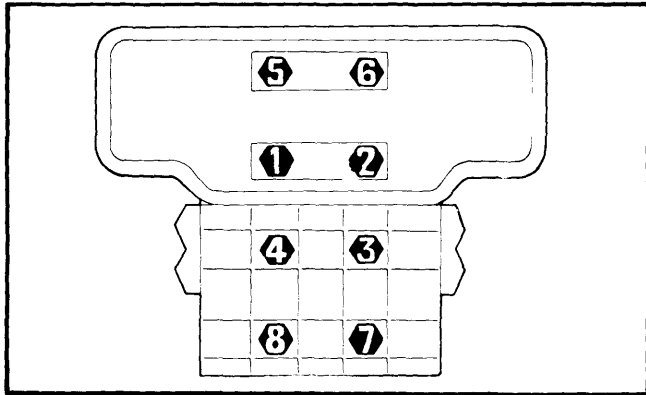
Fig. 7 Tightening Sequence for Main Bearing Nuts
