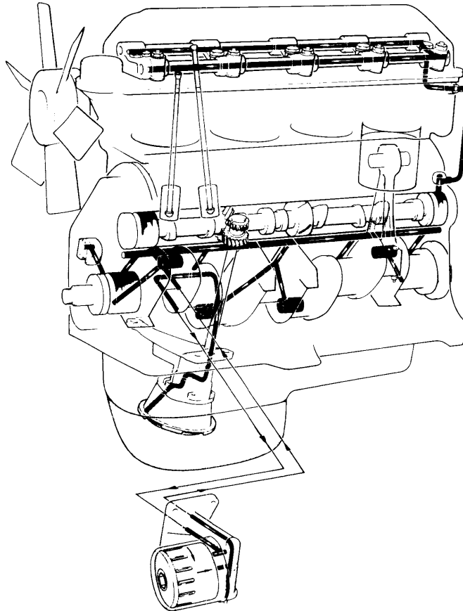
Fig. 13 Sectional View of Peugeot Engine Oiling Circuit with Detail of Components Lubricated
