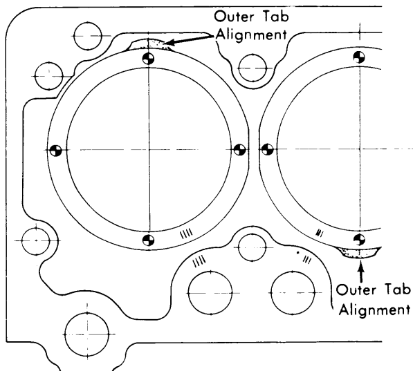
Fig. 8 Fitting Cylinder Liner Gasket to Liner
