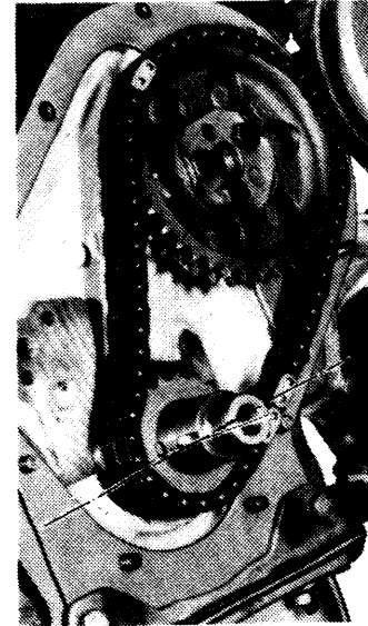
Fig. 11 Correct Position of Crankshaft for Chain Installation
