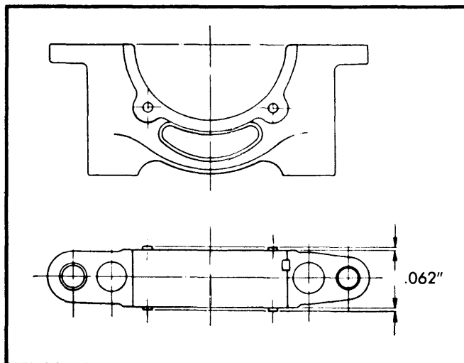
Fig. 5 Detail of Center Main Bearing Cap
