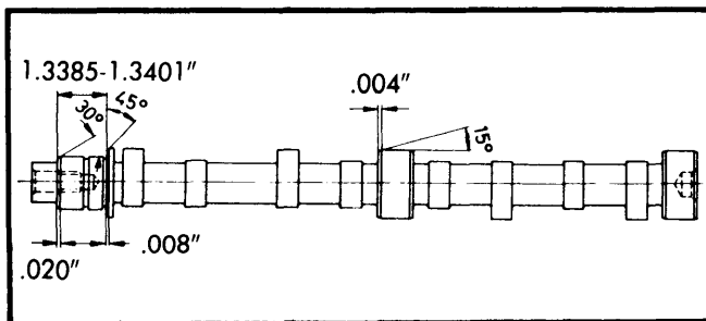
Fig. 7 Detail View of Camshaft
