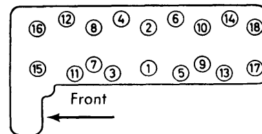
Fig. 1 Cylinder Head Tightening Sequence
