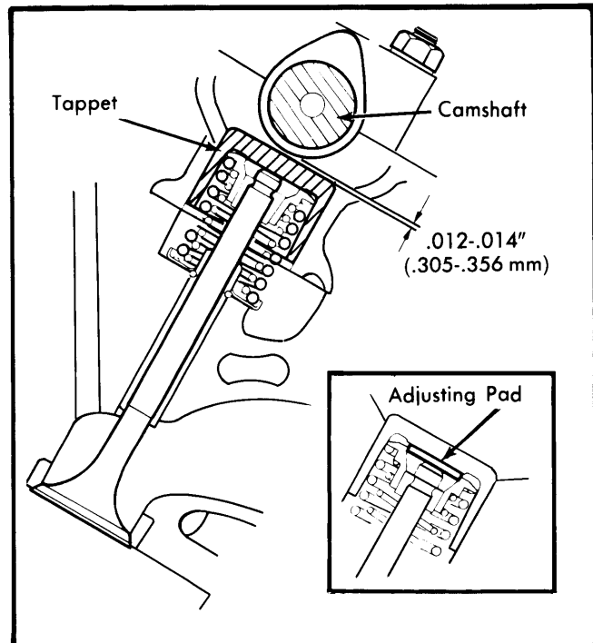
Fig. 5 Correct Valve Tappet Clearance Adjustment Procedure
