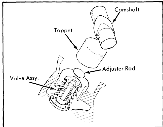
Fig. 4 Expanded View of Valve and Tappet Assemblies
