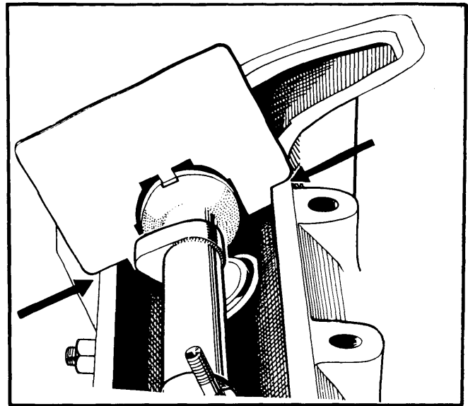
Fig. 16 Valve Timing Guide Inserted in Position
