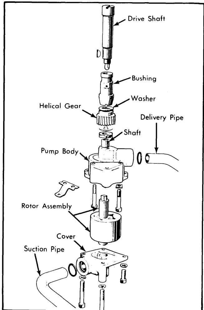
Fig. 17 Exploded View of Jaguar Oil Pump Assembly
