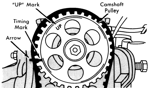
Fig. 5 Camshaft Alignment Marks in Position for Installing Camshaft Belt
