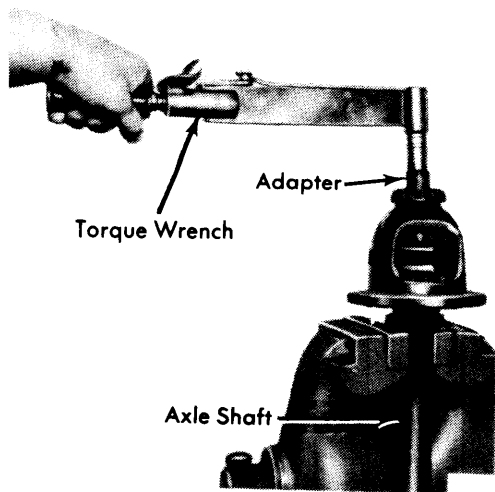
Fig. 6 Measuring Side Gear Torque
