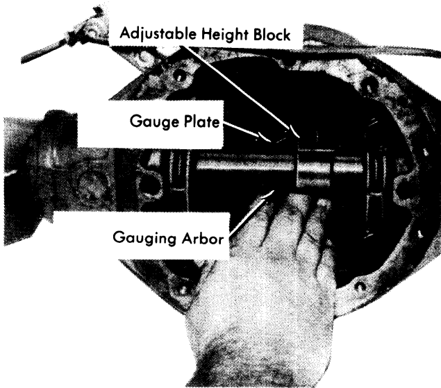
Fig. 3 Gauging Pinion Depth
