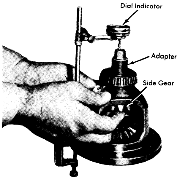
Fig. 5 Measuring Side Gear End Play
