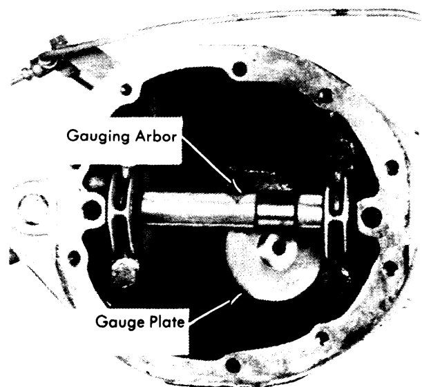
Fig. 2 Pinion Depth Gauging Tools
