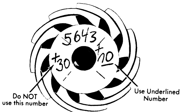
Fig. 4 Pinion Gear Reference Number
