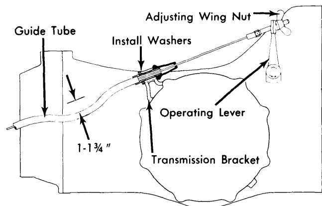
Fig. 1 View Showing Clutch Cable Measuring & Adjusting Points
