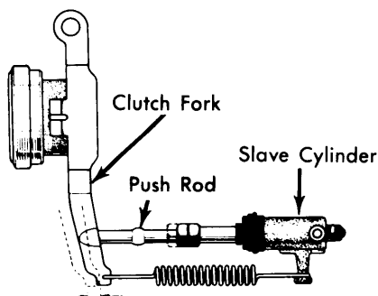
Fig. 6 Clutch Fork Free Play Measurement Location
