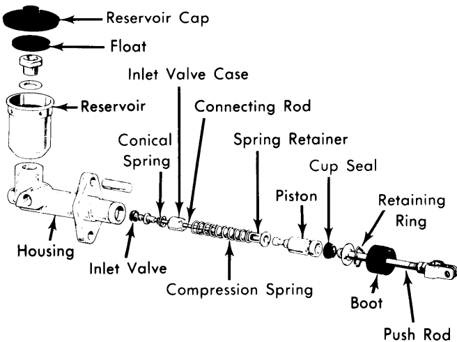
Fig. 3 Exploded View of Clutch Master Cylinder (Corona, Celica, Corolla Shown)
