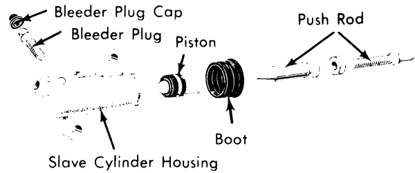
Fig. 4 View of Typical Slave Cylinder — Corona Mk II Shown
