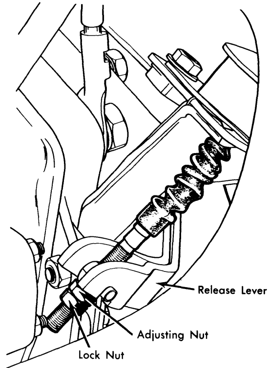
Fig. 3 View Showing Adjustment Point for Clutch Cable
