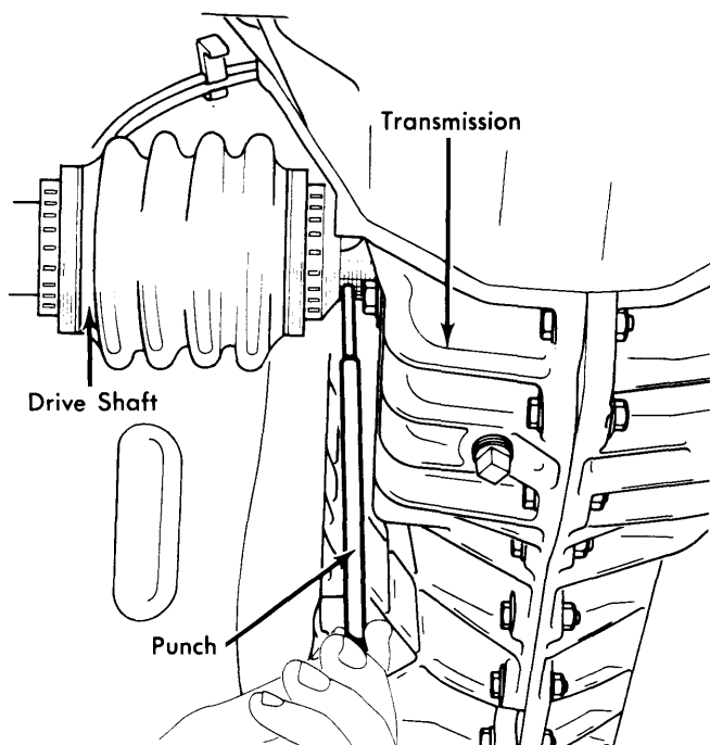
Fig. 1 View Showing Removal of Drive Shaft Roll Pin
