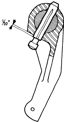
Fig. 2 View Showing Installation Height of Clutch Fork Pin
