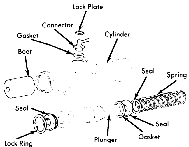
Fig. 2 Exploded View of Clutch Master Cylinder
