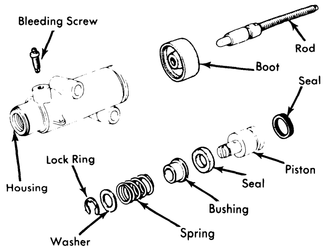
Fig. 3 Exploded View of Clutch Slave Cylinder
