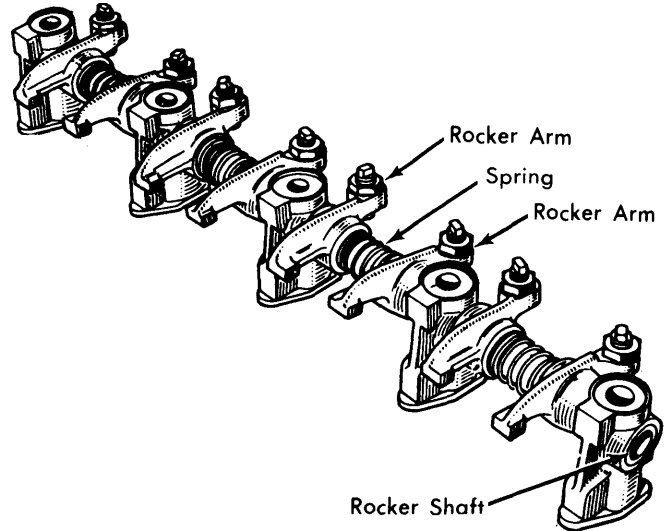
Fig. 2 Renault Rocker Shaft Assembly
