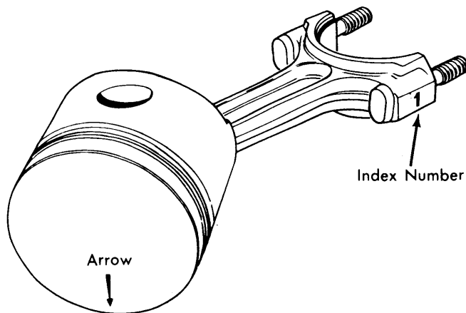
Fig. 6 Piston and Connecting Rod Assembly with Detail of Index Markings
