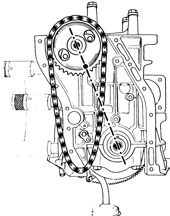
Fig. 10 Camshaft Sprocket Alignment Before Timing
