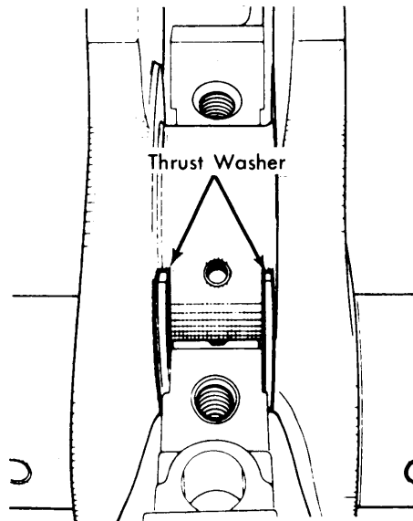
Fig. 7 Crankshaft Thrust Washers in Fitted Position
