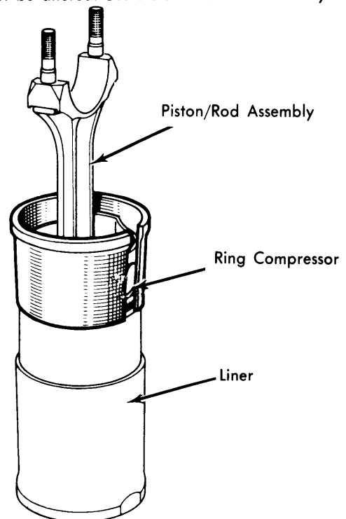
Fig. 4 Inserting Piston into Liner Using Ring Compressor
