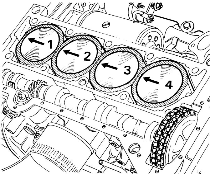
Fig. 3 Showing Cylinder Liners Installed in Block
