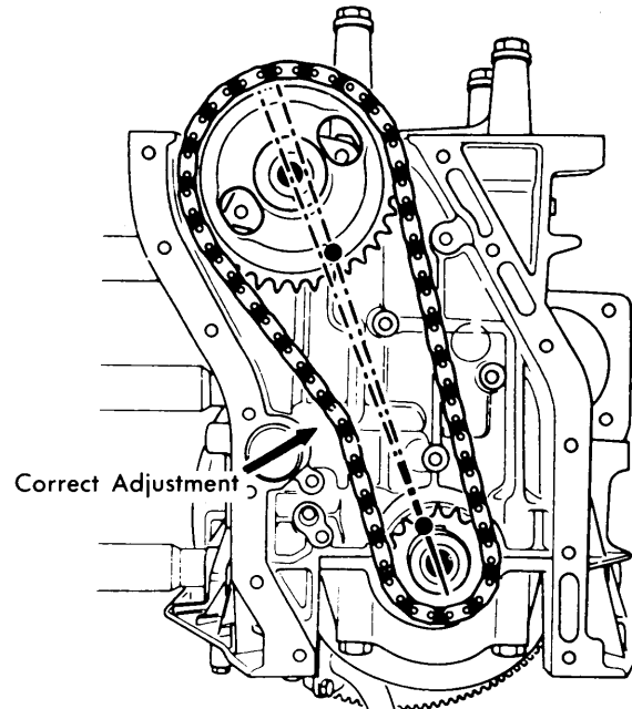
Fig. 12 Camshaft and Crankshaft Alignment with Chain Installed
