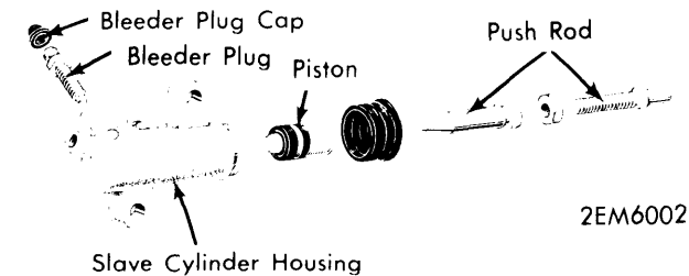
SLAVE CYLINDER COMPONENTS — TYPICAL (CORONA MK II SHOWN)
