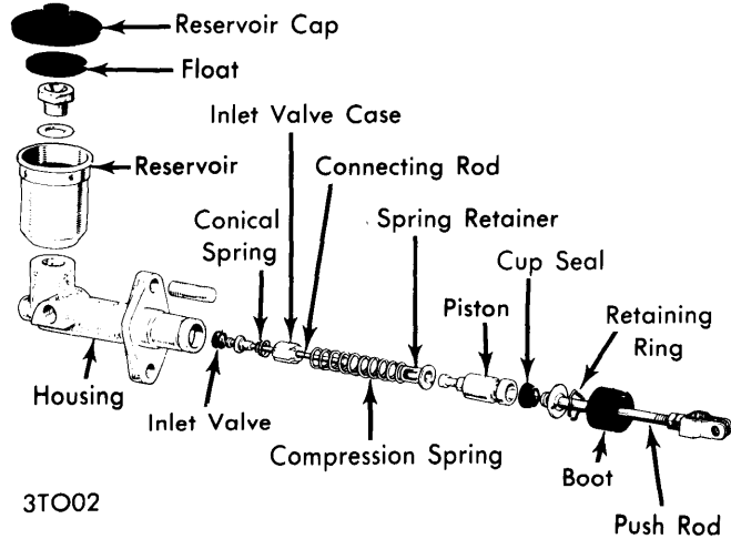
MASTER CYLINDER ASSEMBLY (CORONA, CELICA & COROLLA 1600)
