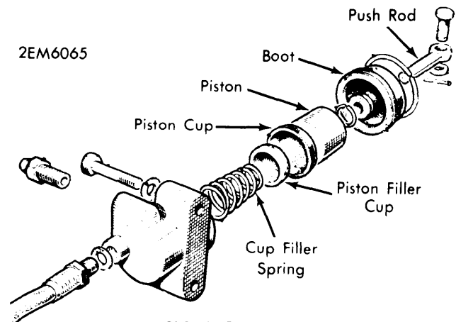
SLAVE CYLINDER
