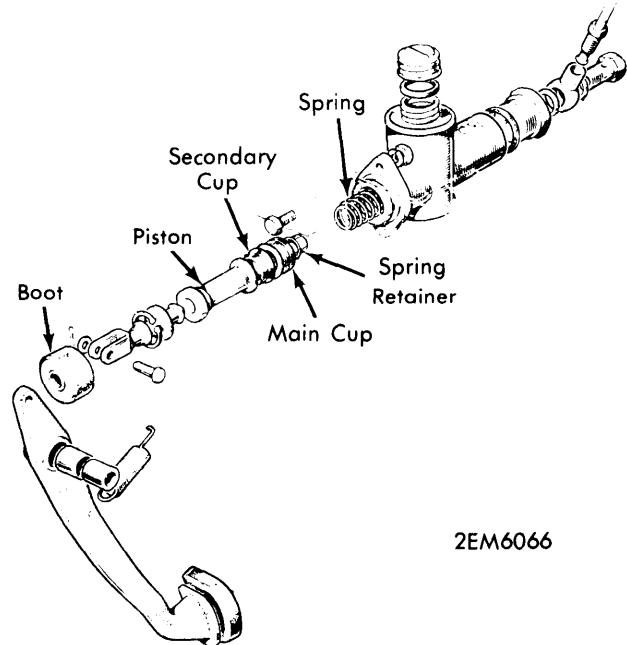
CLUTCH MASTER CYLINDER
