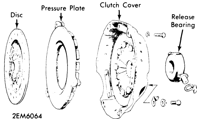
CLUTCH ASSEMBLY
