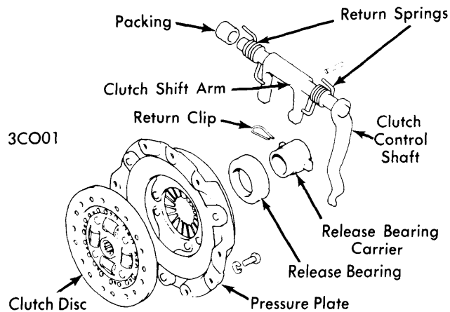
CLUTCH ASSEMBLY
