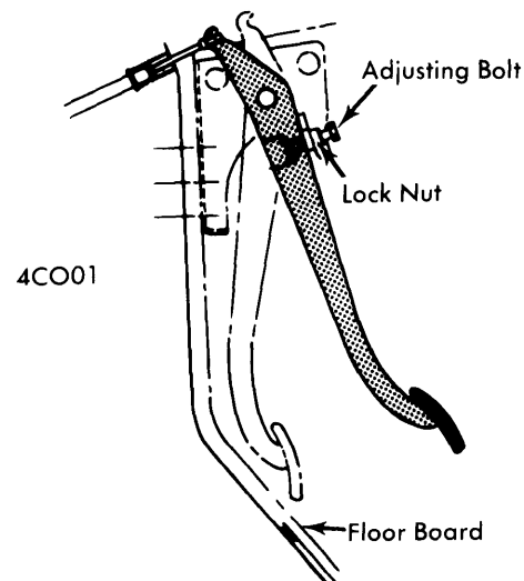
CLUTCH PEDAL ADJUSTMENT
