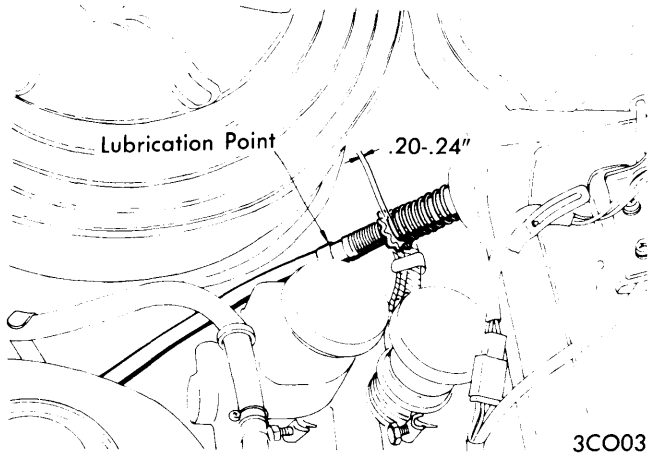
CLUTCH CABLE ADJUSTMENT
