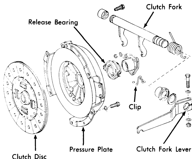
CLUTCH ASSEMBLY
