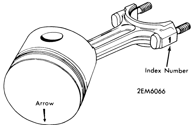
PISTON ASSEMBLY
