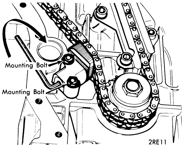
TIMING CHAIN — CORRECT ADJUSTMENT
