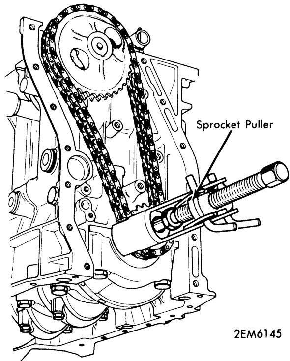
CRANKSHAFT SPROCKET REMOVAL
