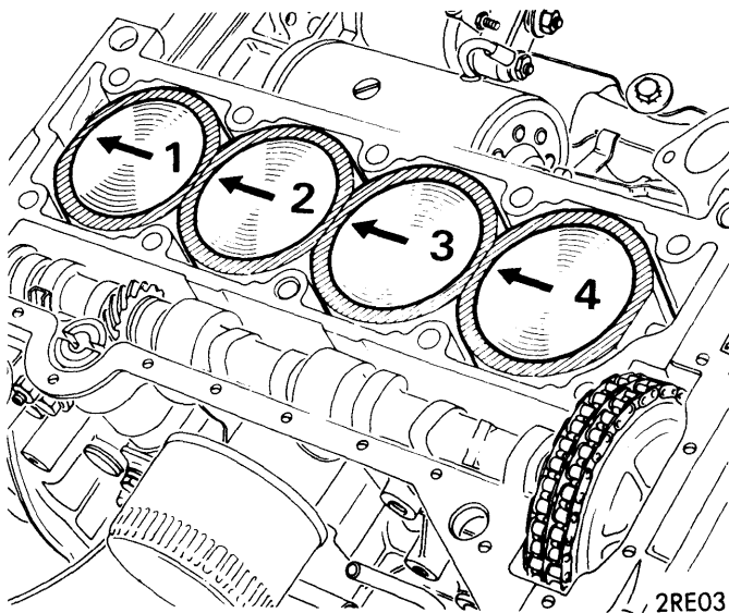
LINER INSTALLATION
