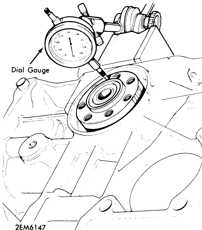
MEASURING CRANKSHAFT END PLAY
