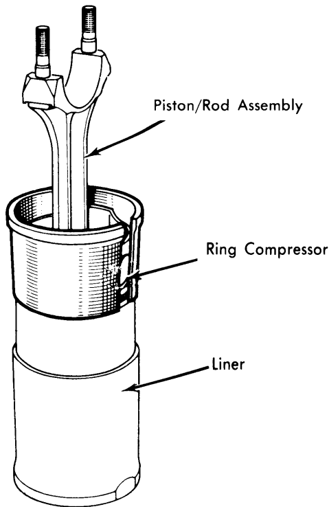
PISTON INSTALLATION
