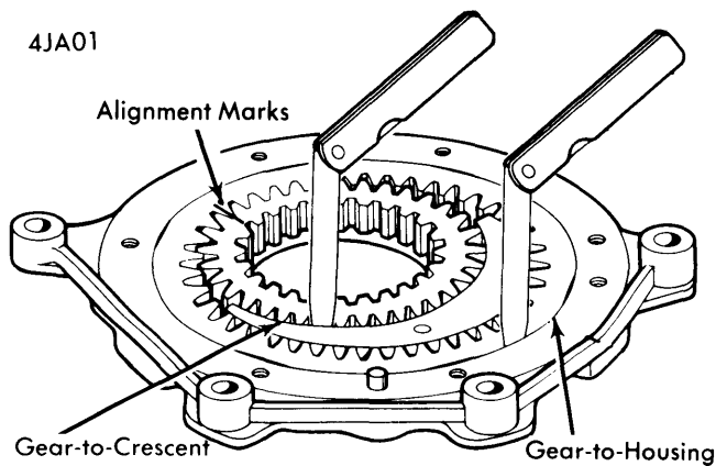
MEASURING OIL PUMP CLEARANCES
