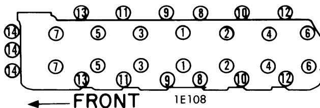
V12 CYLINDER HEAD TIGHTENING SEQUENCE
