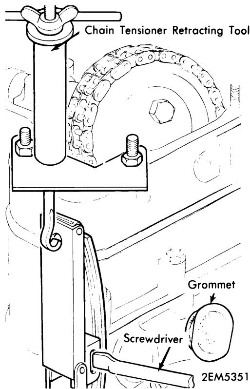
TENSIONER RETRACTING TOOL
