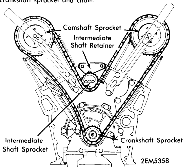
TIMING CHAIN REMOVAL
