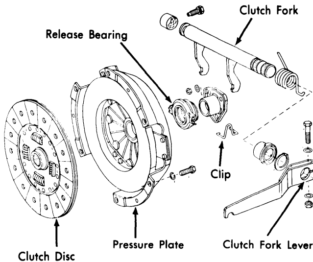
CLUTCH ASSEMBLY
