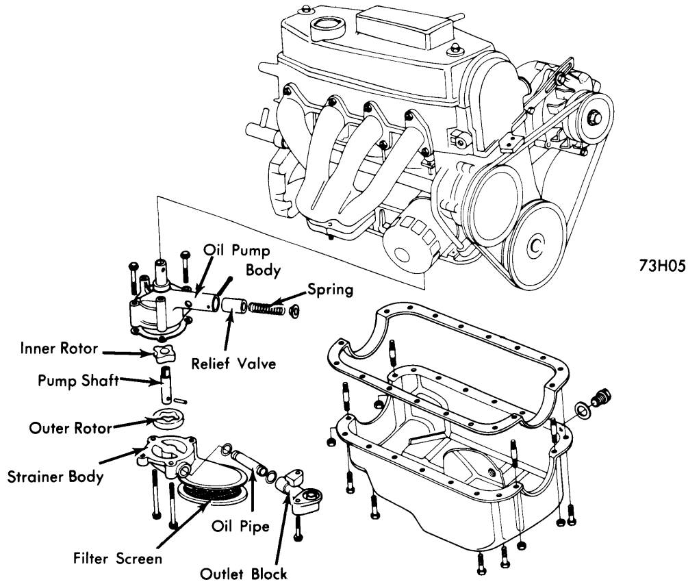
OIL PUMP & PAN ASSEMBLY
