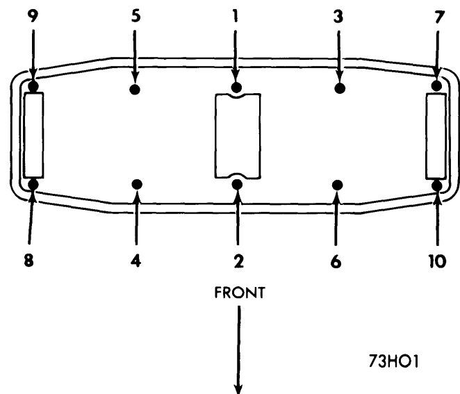
CYLINDER HEAD TIGHTENING SEQUENCE
