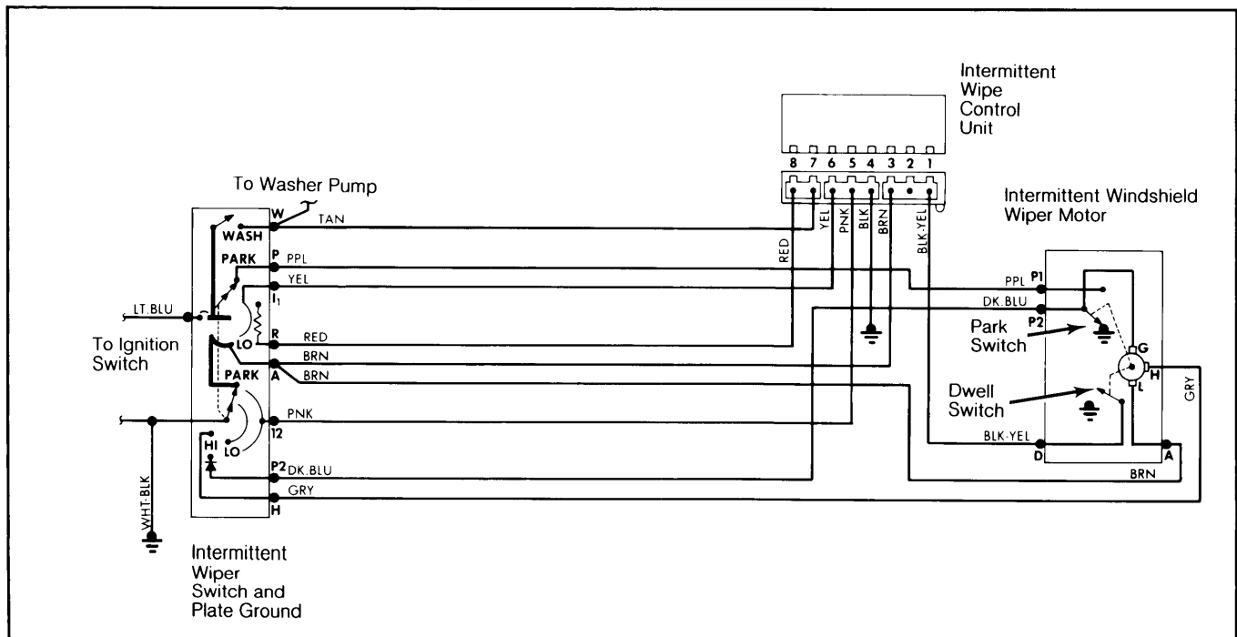
Fig. 3: Chrysler Intermittent Wiper Wiring Diagram
