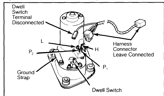
Fig. 1: Two Speed Intermittent Wiper Motor Terminals
