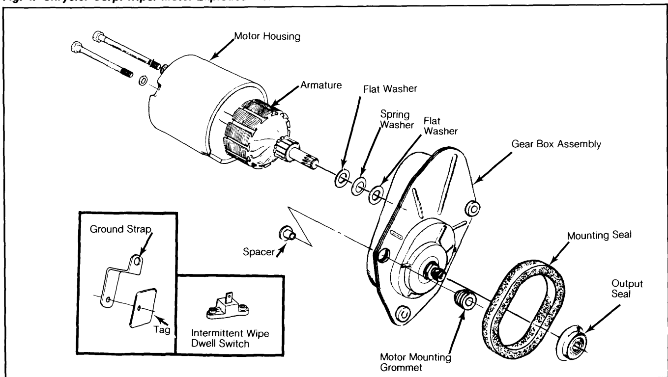
Fig. 4: Chrysler Corp. Wiper Motor Exploded View
