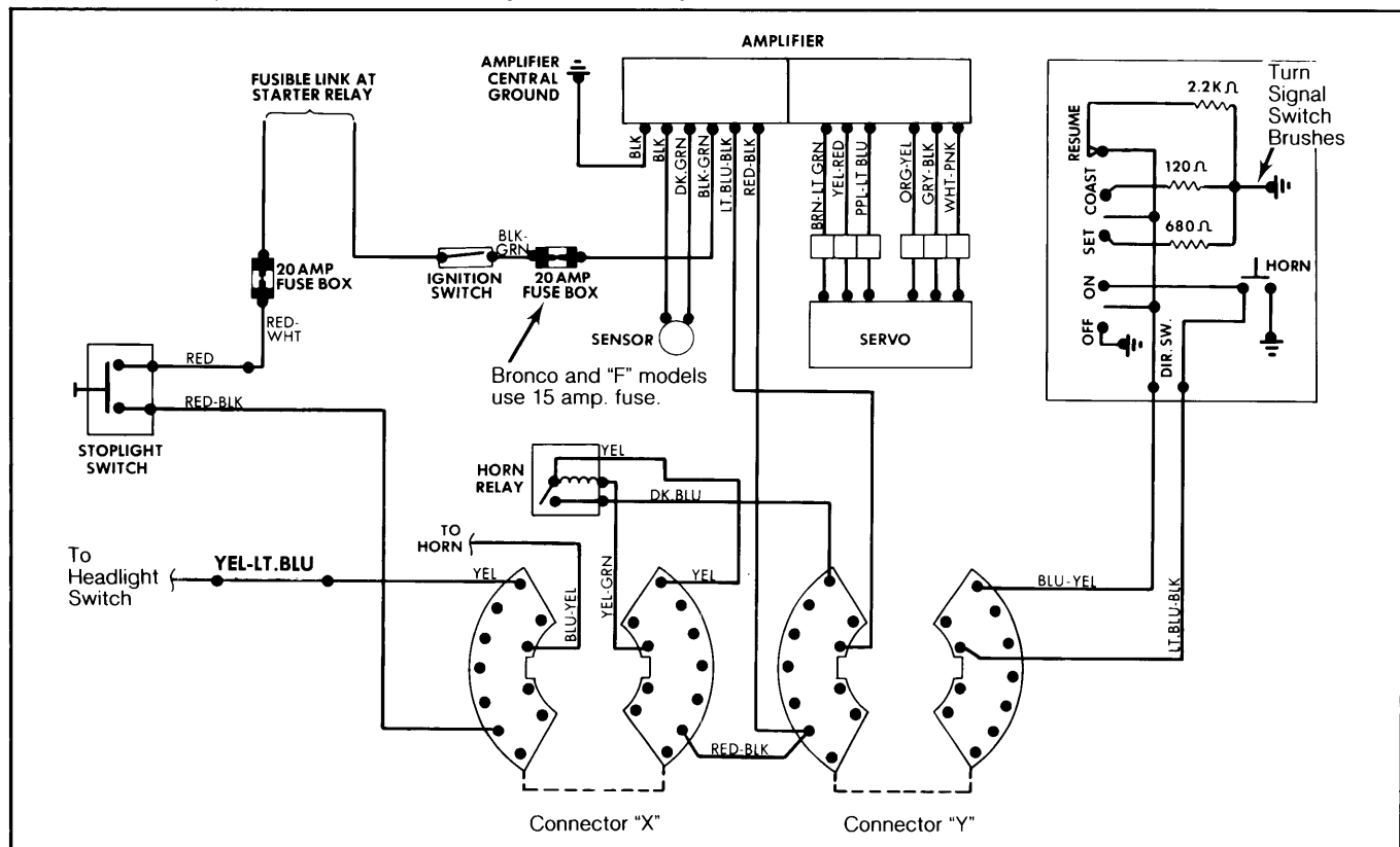
Fig. 2: Wiring Diagram of Ford Automatic Speed Control System
