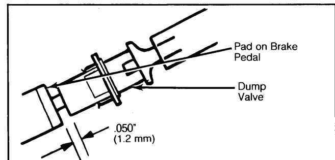
Fig. 3: Vacuum Dump Valve Adjustment
