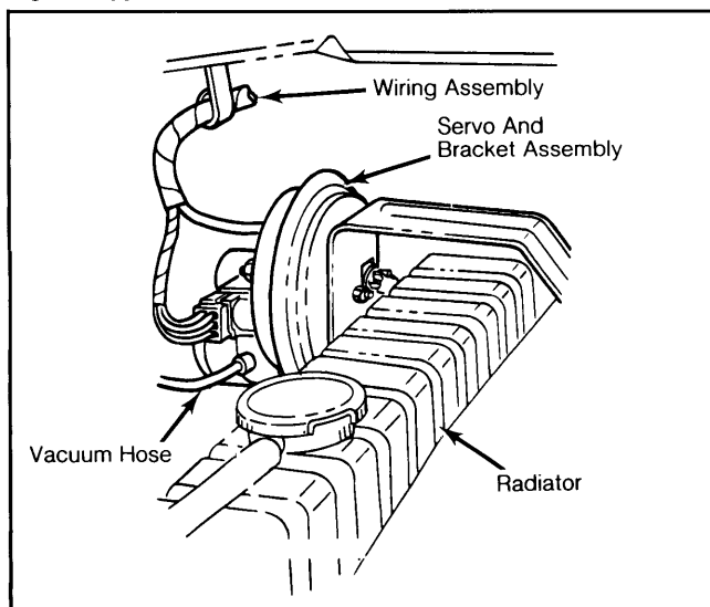
Fig. 1: Typical Servo and Bracket Installation
