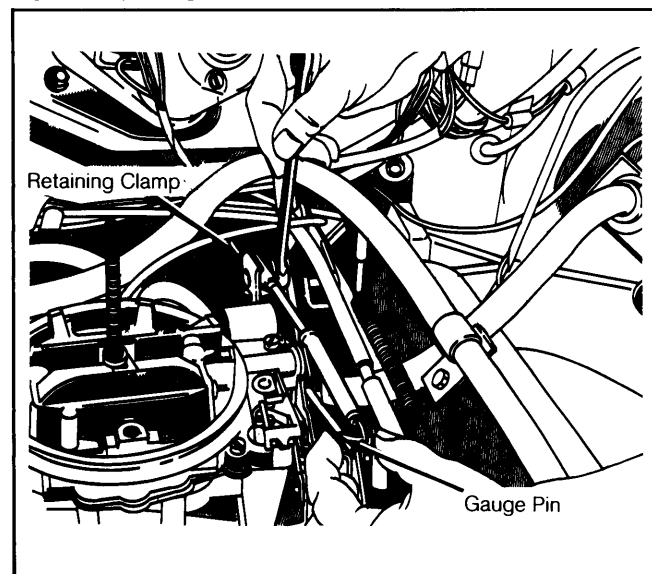
Fig. 2: Adjusting Servo Throttle Cable
