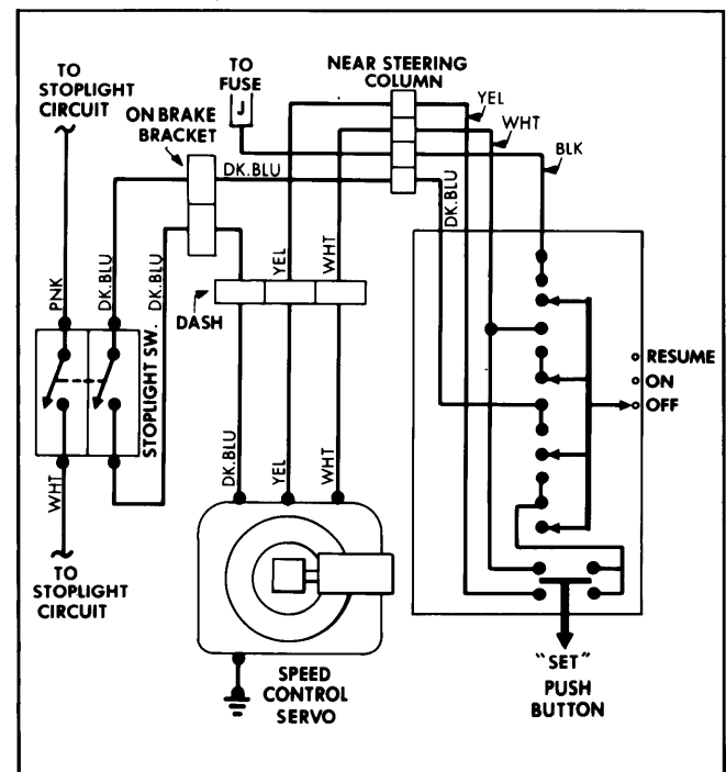
Fig. 1: Wiring Diagram of Chrysler Corp. Speed Control System
