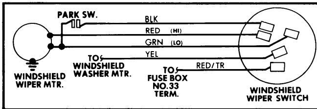
Fig. 1 Jeep 2-Speed Wiper System Wiring Diagram ("CJ" & Scrambler Models)
