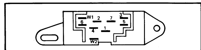
Fig. 7 Blade Type (Slide Switch) Connector Non-Interval
